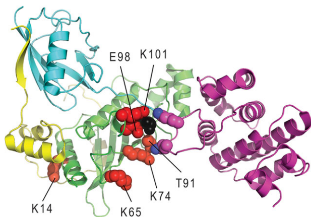
FIGURE 2 Advantageous growth mutations. The Ubc9 (green cartoon) structure complex (PDB: 3uiu) bound to RanGAP1 (magenta cartoon), SUMO2 (cyan cartoon), and the E3 ligase IR1 domain of RanBP2 (yellow cartoon) highlights positions of residues with advantageous growth mutations (red spheres, labeled according to WT position) with respect to the active site Cys (black sphere) and the consensus substrate tetrapeptide E and K residues (magenta spheres)
